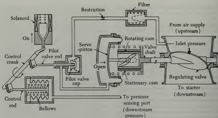
FIGURE 5-18. Pressure-regulating and shutoff valve in "on" position.
